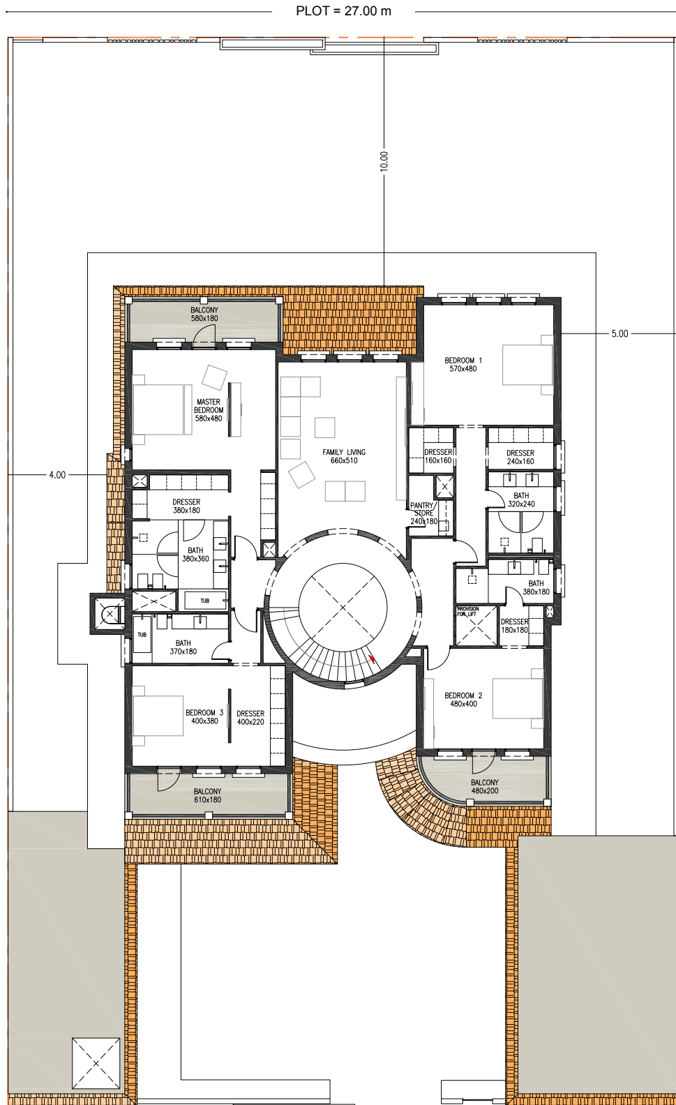
First Floor
